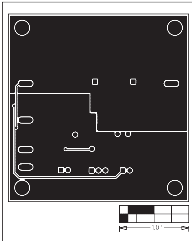
Figure 4. MAX15020 EV Kit PCB Layout—GND Layer 2
